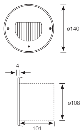
Flush-mounting dimensions: 101 mm x ø 108 mm
